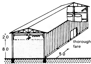
3 Hay storage barn with overhead loader
